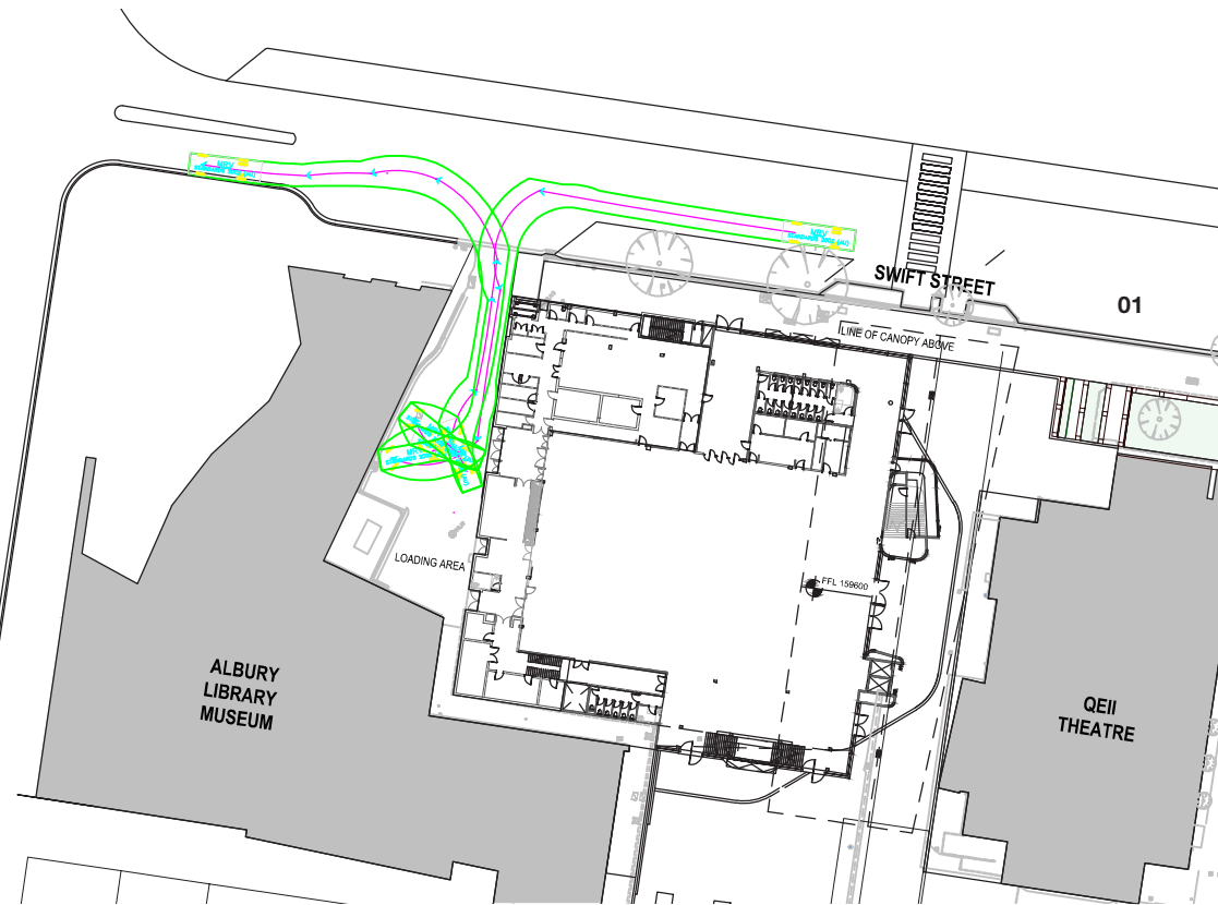
Option 04 - Medium Rigid Vehicle (MRV) forward entry and exit (method 1), from and to, westbound lane.
